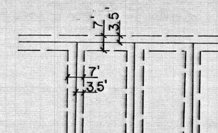
TYPICAL EASEMENT
