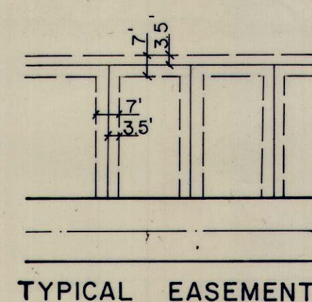
TYPICAL EASEMENT
